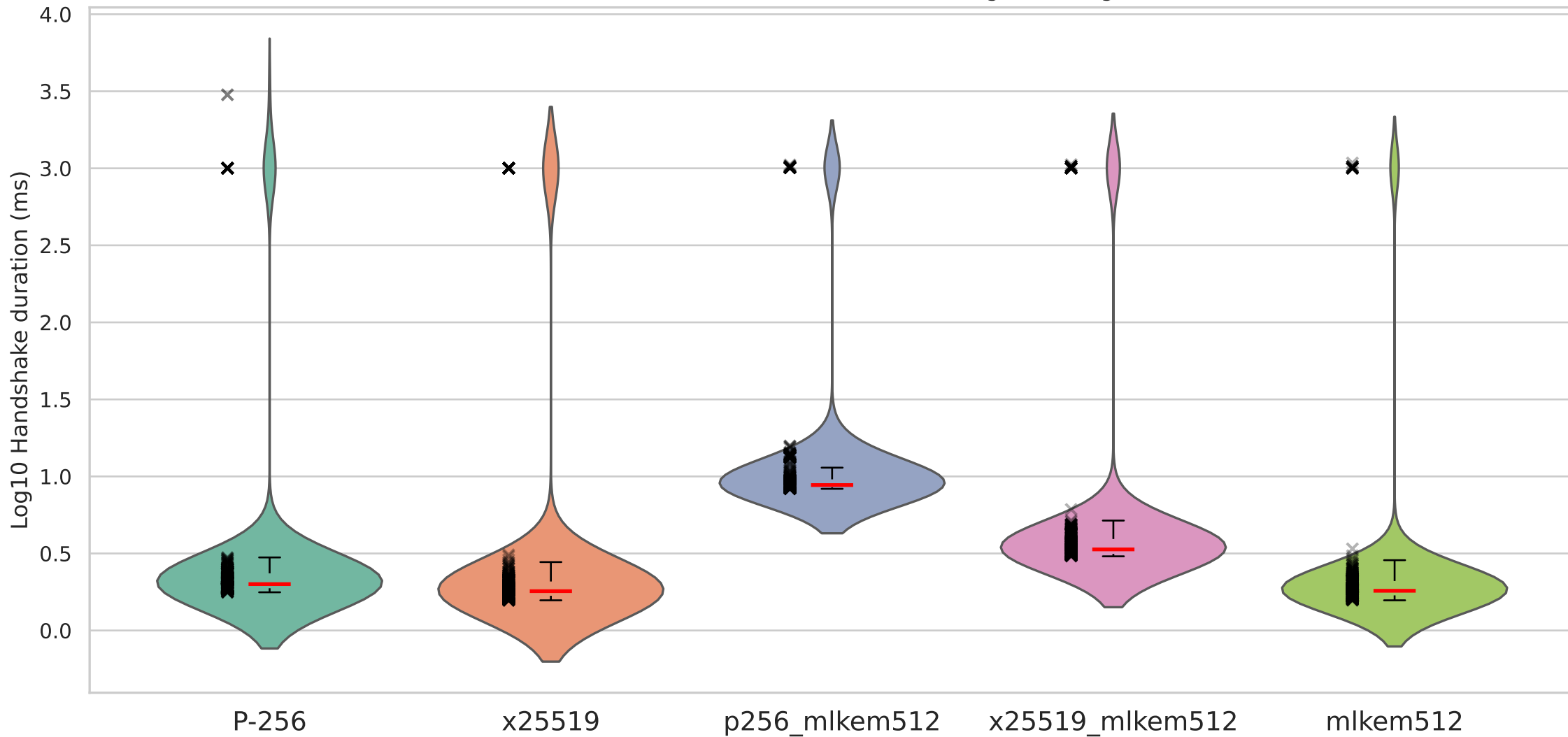
Handshake duration on QUIC with ed25519 signature algorithm
